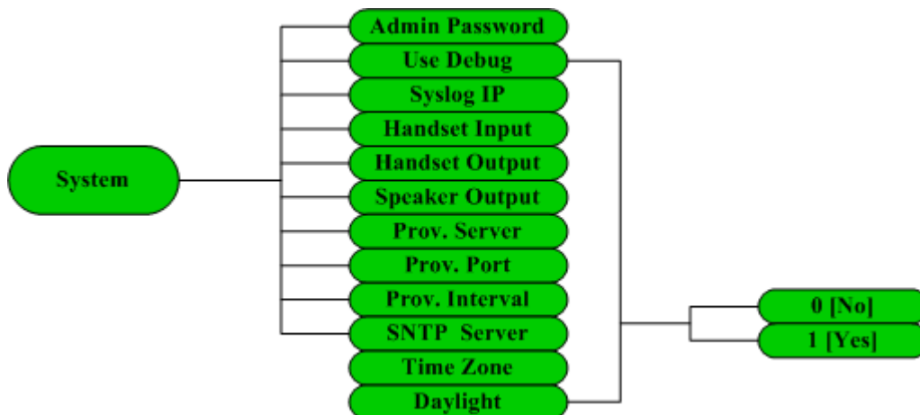
Fig 5.1.6 System submenu
